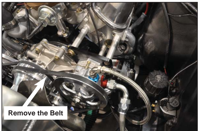
Remote reservoir version of power steering pump shown.
